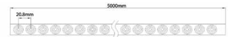
-LED STRIP 24V 18W/m with OPTICS 20° x 45°
