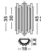
FELIX - 9287917 Gold Aluminium & Acrylic LED 20 Watt 220 - 240 Volt 1472Lm 3000K IP20 D: 18 W: 8.8 H: 50 cm
