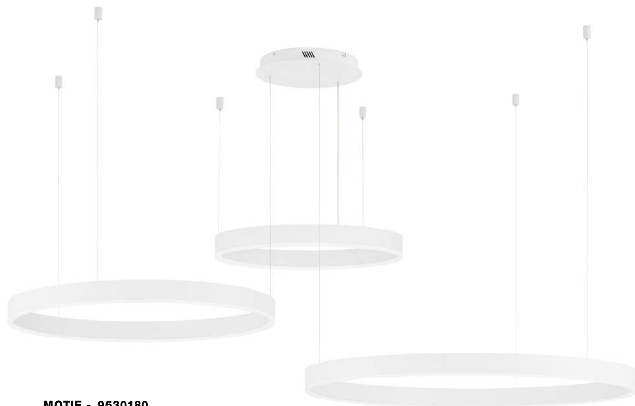
MOTIF - 9530180 Dimmable Sandy White Aluminium & Acrylic LED 40/48/55 Watt 230 Volt 13163Lm 3000K IP20 D1: 60 D2: 80 D3: 100 H: 250 cm LED WARM WHITE DRIVER INCL.
