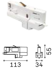
TRACK ADAPTOR
